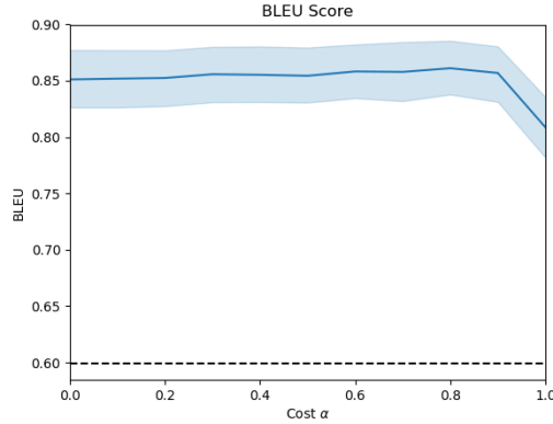
Fig. 8. BLEU score vs cost \alpha for MTurk dataset. Dotted line shows BLEU score for unmodified prompts.
