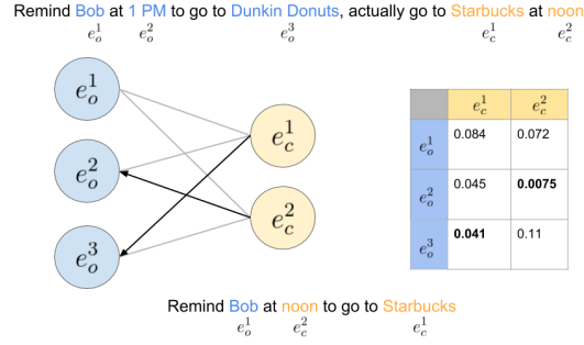
Fig. 5. Entity matching and replacement formulated as a minimum cost assignment problem. Here, an example of the entity matching is shown with multiple parameters and replacement candidates. Table represent costs between replacements, and the assignment with the least cost is used to generate the output.
