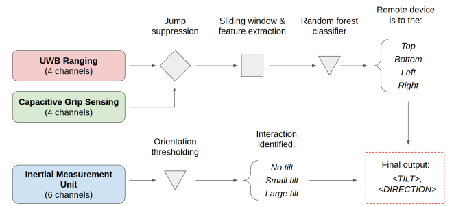
Figure 6: Sensor processing block diagram.
