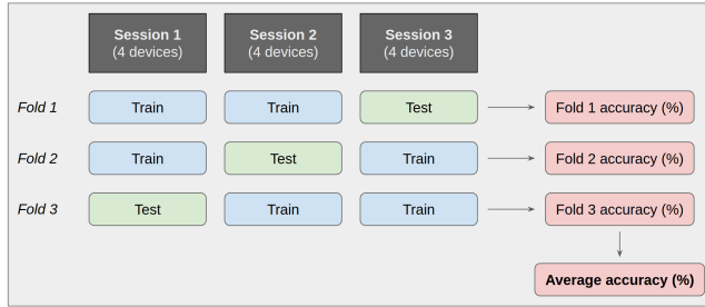
Figure 12: Cross-validation evaluation scheme for training and testing AdHocProx’s machine learning models.
