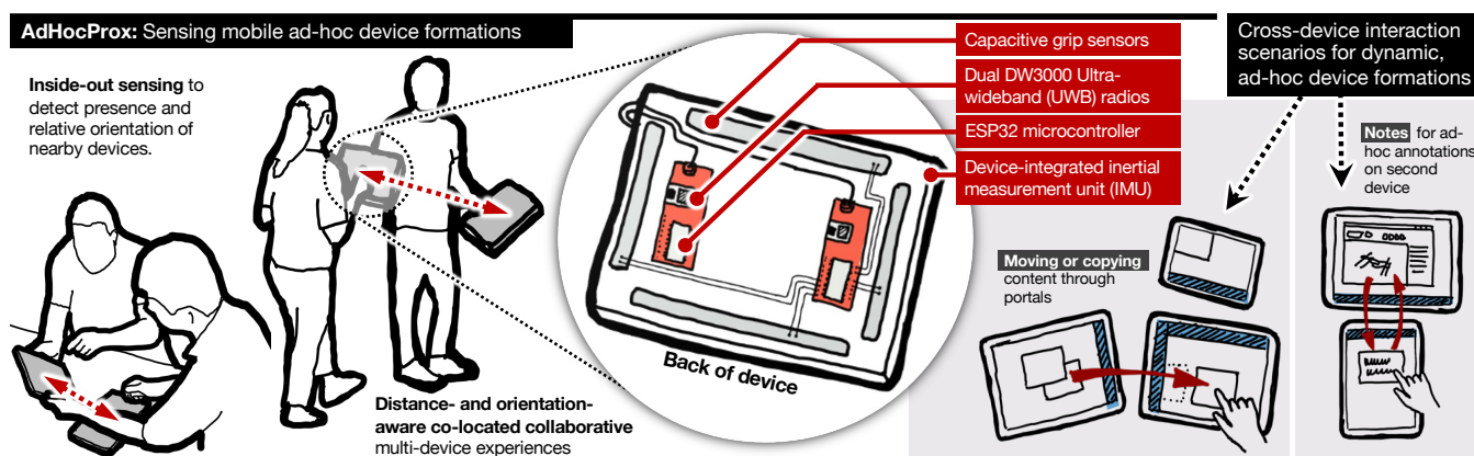
Figure 1: AdHocProx leverages multiple inside-out sensing modalities (including dual Ultra-Wideband radios, capacitive grip sensing, and fused inertial orientation) built into a device such as a tablet to detect presence, relative position, and device-motion gestures towards other nearby mobile devices. AdHocProx achieves this without recourse to externally-anchored beacons, central orchestration, or even reliance on local WiFi connectivity. This unlocks a number of cross-device interaction scenarios for highly dynamic, ad-hoc device formations outside of infrastructure-heavy “smart room” or lab settings.
