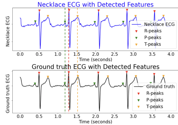
Figure 15: An example of synchronized ECG signals obtained from the ECG necklace and the ground truth device, with the P, R, and T waves identified by the NeuroKit2 Python tool.
